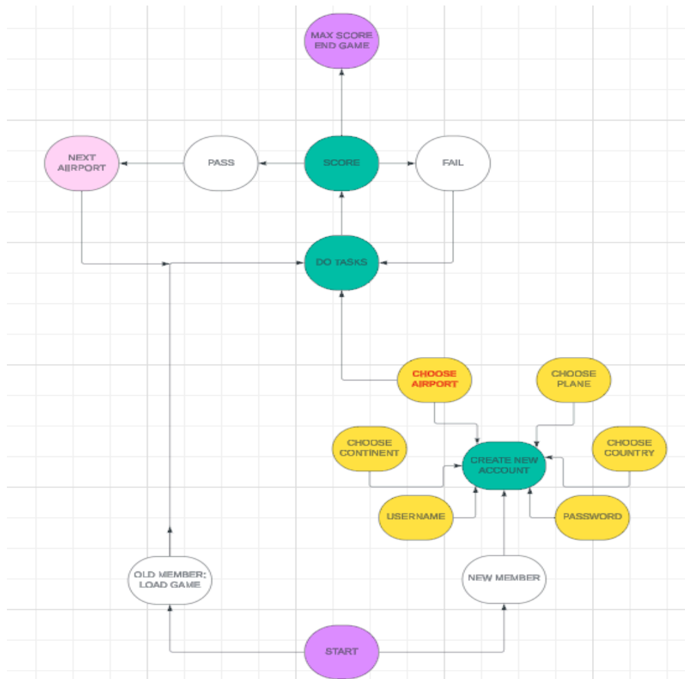
Figure 1: Game flowchart
